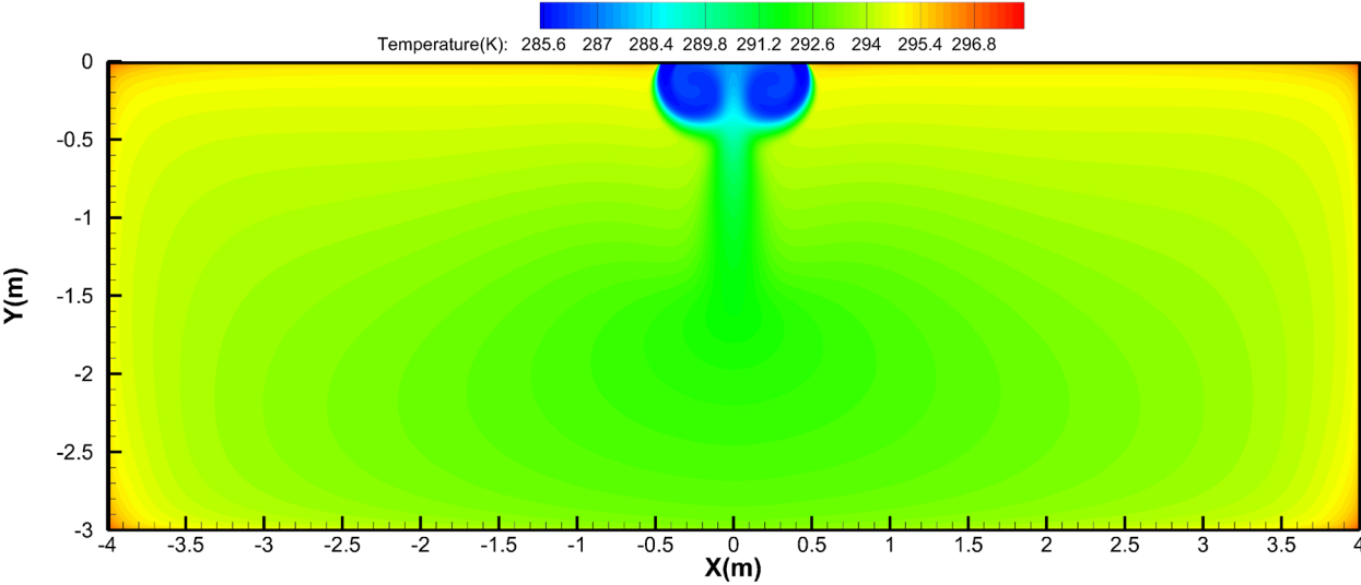
Cooling temperature distributions
